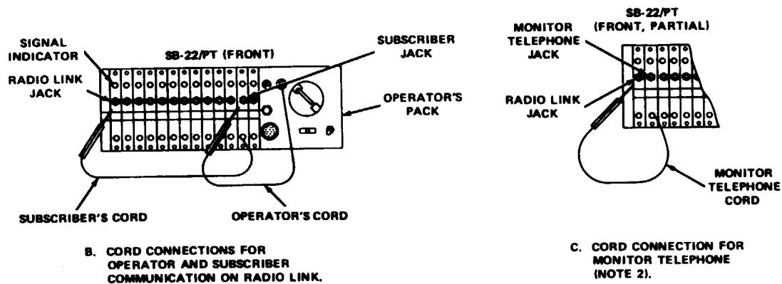
Figure 6-16. Radio Set Control AN/GSA-7 with RT-841/PRC-77 to Provide RWI; Connections and Control Settings.
